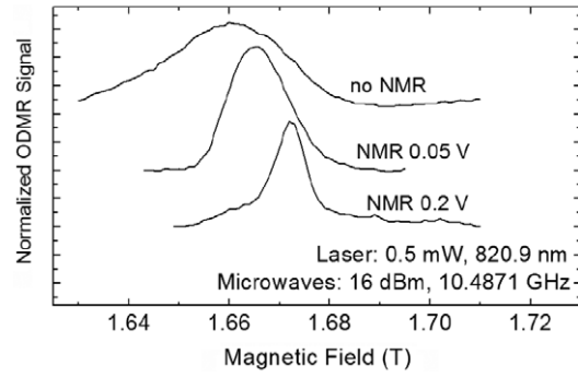
Fig. 4. Bulk sample ODMR peaks with varying NMR powers (function generator voltages shown). With sufficient rf (bottom curve), the dynamic nuclear polarization could be eliminated, shifting the ODMR peak back to its equilibrium position. Peaks are vertically offset for clarity.
