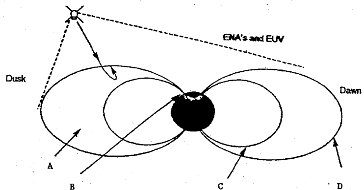
Figure 1. View of the IMAGE satellite relative to the Earth. A. Detached plasma region, B. Simultaneous Auroral Image, C. Plasmapause (disturbed times), D. Plasmapause (quiet times).
