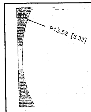
Figure 2. Side view drawing of the EUV mirror. The mirror has a diameter of 12.9 cm and a radius of curvature of 13.52 cm.
