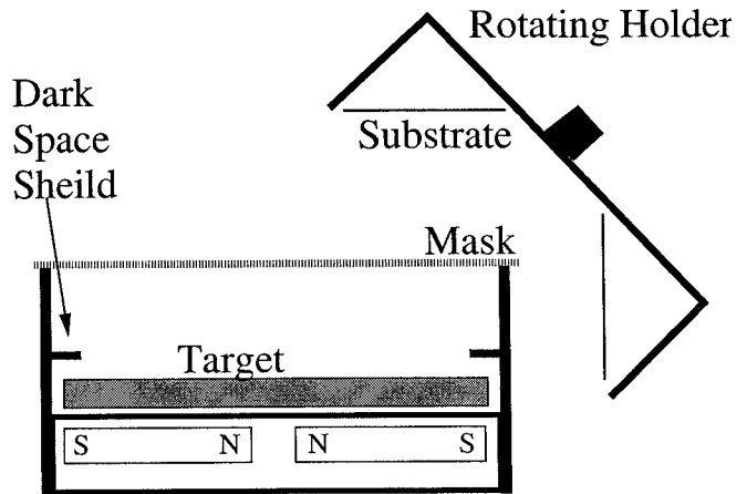
Figure 5. Schematic of rotating sample holder relative to sputter gun (size and angle are not to scale).
