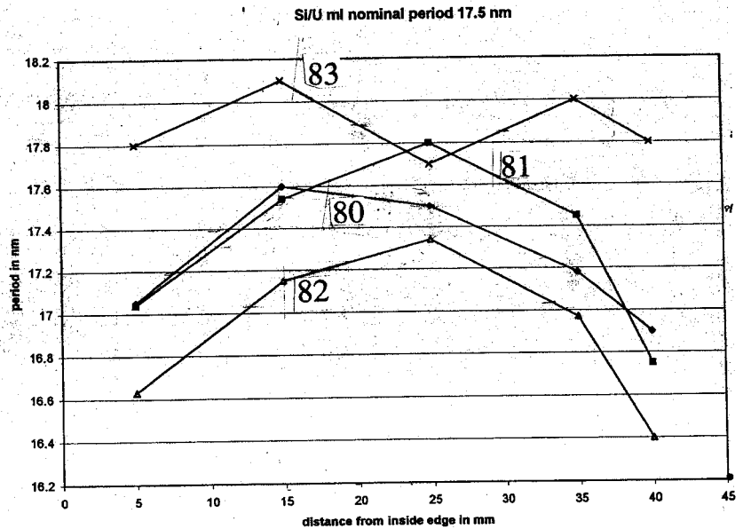
Figure 4. Uniformity: The multilayer period as a function of distance from the inside edge of the mirrors as measured by XRD on Silicon wafer flats. The tilt angle of the spindle spinning the mirrors is 16.4 degrees from normal. The deposition times were the same for all four multilayers. As can be seen the period falls off at higher radii for 80,81,82. Most of this decrease is removed ( sample 83) when the outer edge of the mask is cut off.( see Figure 2 of Squires 1999).
