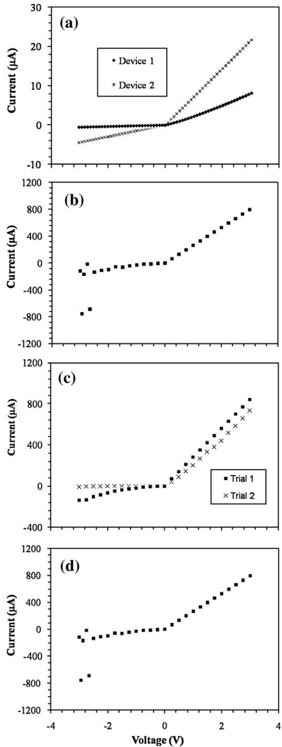
Fig. 4. Electrical characterization of (a) devices 1 and 2; (b) device 3, (c) device 4, and (d) device 5. On/off ratios of devices 1 and 2 were 20 and 5, and maximum current capacities 8 \mu\text{A} and 22 \mu\text{A} , respectively. On/off ratios of device 3 was 27 and maximum current capacity 679 \mu\text{A} . On/off ratios of 6 and 108, and maximum current capacities of 841 and 735 \mu\text{A} were obtained from two subsequent trials performed with device 4. Finally, on/off ratio of device 5 was difficult to determine because of the dramatic variations in the reverse-bias region; the maximum current capacity is 794 \mu\text{A} .
