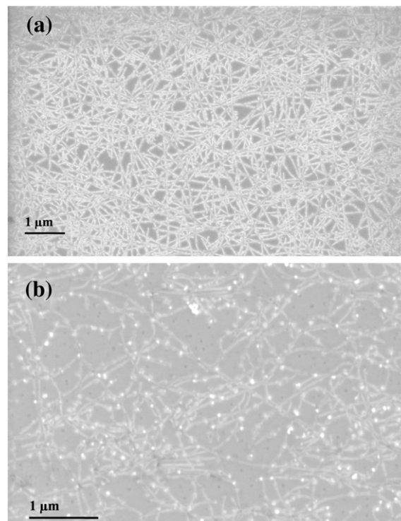
Fig. 1. SEM micrograph of carbon nanotube network used to fabricate (a) devices 1 and 2 and (b) devices 3, 4, and 5, in which significantly lower density of nanotubes and large iron particles are found. Note that the in-lens configuration of the SEM is known to highlight nanotubes but their width is not well represented in the image.
