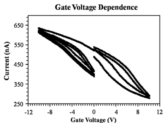
Fig. 5. Gate voltage dependence of diode device 1 (Fig. 1a).
