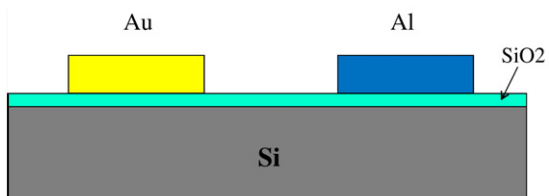
Fig. 3. Cross section of final device. The nanotube mat is not pictured but is a thin layer on top of the SiO 2 layer and beneath the Au and Al contacts. There are two modes for making electrical measurements using this structure. In the first mode, Au and Al electrodes (source–drain) are contacted and current is measured as the source–drain voltage is varied. In the second mode the underlying silicon is contacted and acts as a gate, setting up an electric field which depletes or injects current carriers into the nanotubes depending on its bias.
