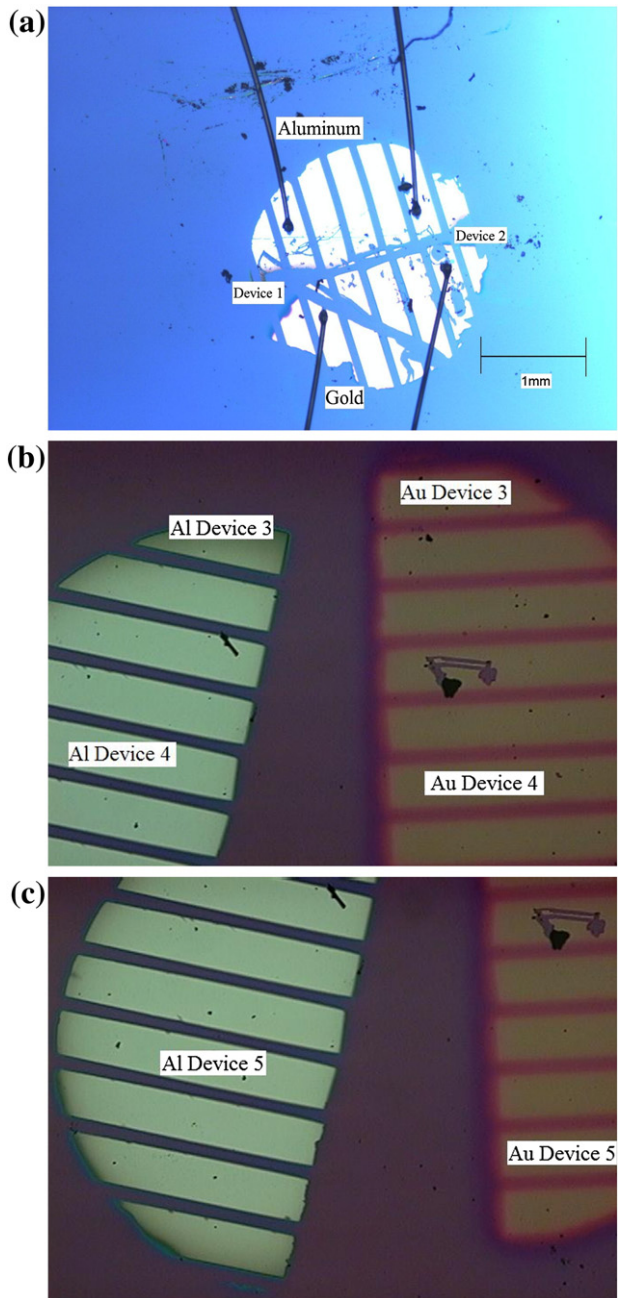
Fig. 2. Devices (a) 1 and 2, (b) 3 and 4, and (c) 5 are pictured. Al and Au electrodes are identified. The mat of nanotubes covers the entire pictured area and is below the deposited electrodes. Note the variation in spacing between the electrodes of the different devices.
